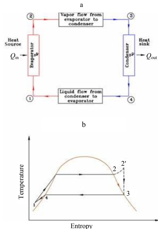
Fig. 2. Heat Pipe Thermodynamic Diagram [12]:
