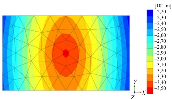
Total displacements u_z (scaled up 200 times)
